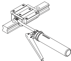
Fig.1 Lubrication Using a Grease Gun
